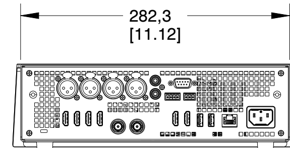
REAR VIEW
